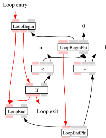
Fig. 5 Graph for a loop counting from 0 to n-1.
