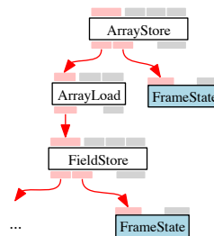
Fig. 9 Simple example using two frame states.
