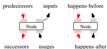
Fig. 1 A node and its edges.
