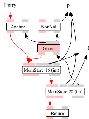
Fig. 14 After removing the frame states.
