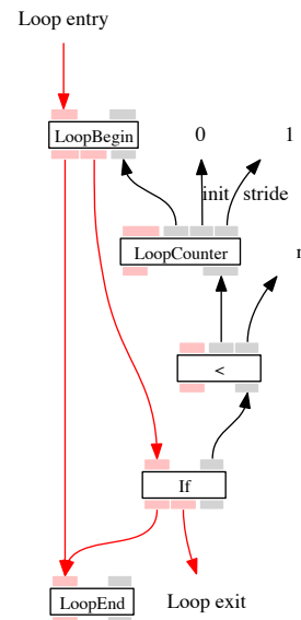
Fig. 6 Graph after loop counter transformation.
