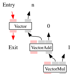
Fig. 8 Graph after vectorization.
