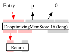
Fig. 16 Fully optimized method.
