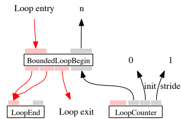
Fig. 7 Graph after bounded loop transformation.
