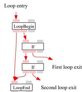
Fig. 4 A simple loop with two exits.
