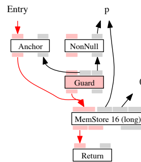
Fig. 15 After coalescing the two memory stores.
