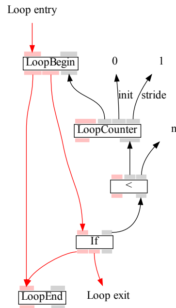
Fig. 3 Graal compiler graph after loop counter transformation.
