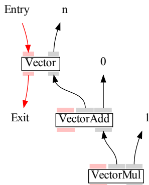
Fig. 5 Graal compiler graph after bounded loop transformation.
