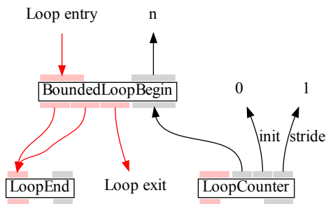
Fig. 4 Graal compiler graph after bounded loop transformation.
