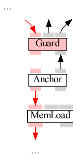
Fig. 11 A guard that is fixed to the control flow using an anchor instruction.
