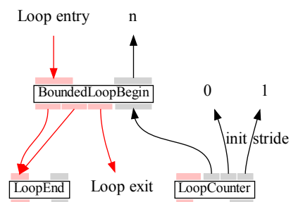
Fig. 4 Graal compiler graph after bounded loop transformation.
