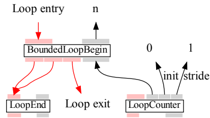
Fig. 5 Graph after bounded loop transformation.
