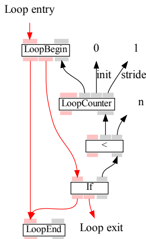
Fig. 4 Graph after loop counter transformation.
