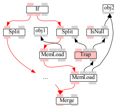
Fig. 8 A load guarded by a null check trap.
